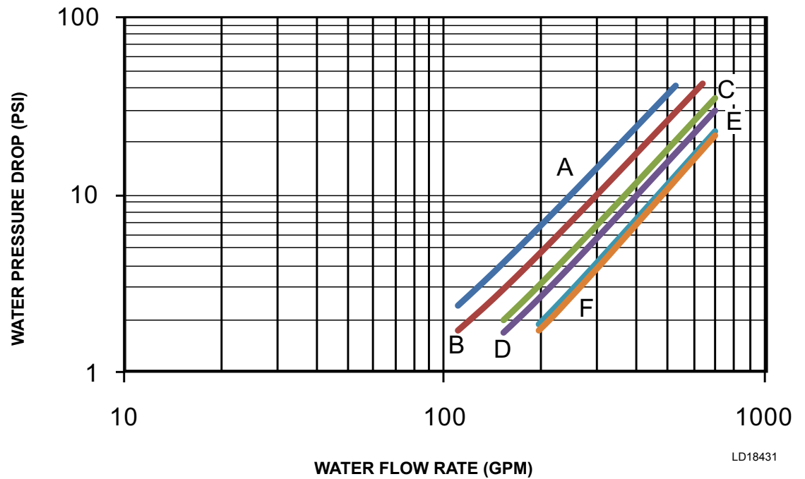
QTC3 EVAPORATOR PRESSURE DROP CURVE
